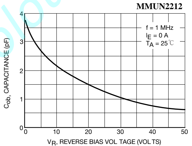
Figure 4. Output Capacitance
