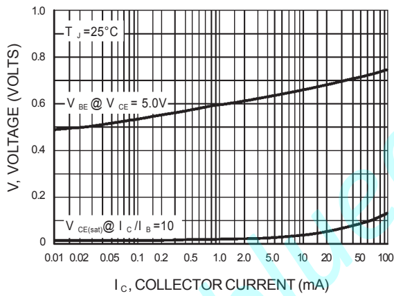
Fig 9. "On" Voltages
