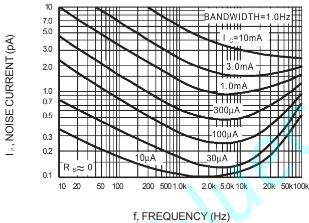
Fig 4. Noise Current
