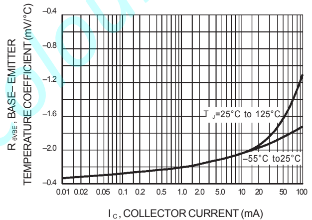
Fig 10. Temperature Coefficients
