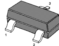
1.Base (IN) 2.Emitter (GND) 3.Collector (OUT) SOT-23 Plastic Package
